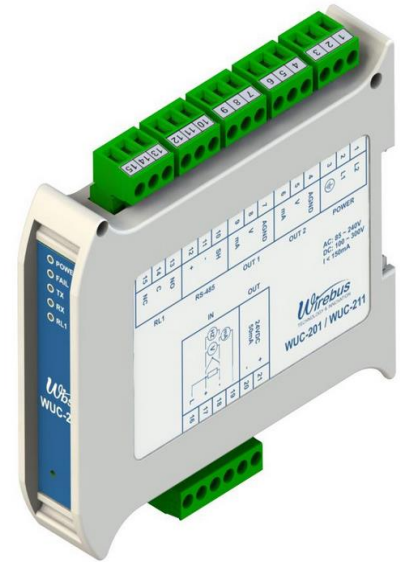
Figura 1 – Conversor WUC-211
