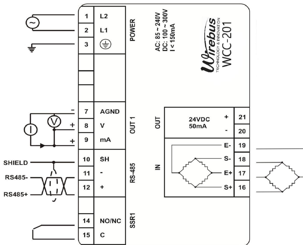
Figura 5 – Borneiras WCC-201/DC
