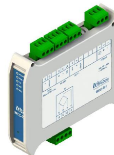
Figura 1 – Conversor WCC-201
