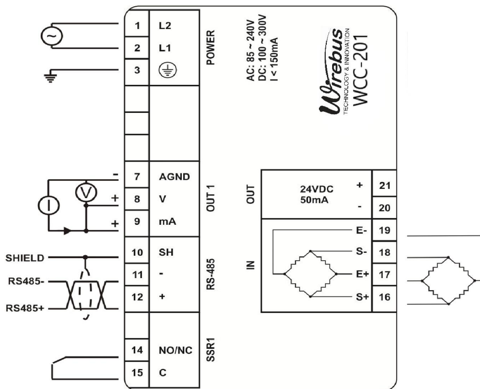
Figura 4 – Borneiras WCC-201/AC
